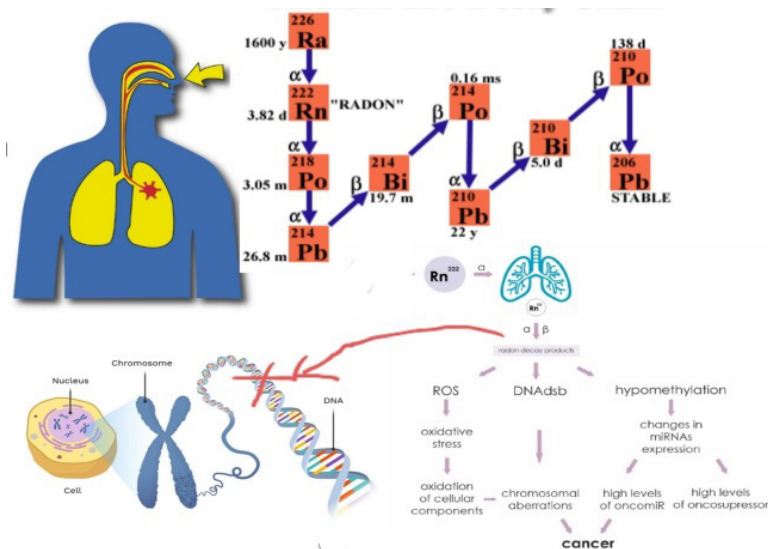
Fig. 1. Radon particles could enter a human body and decay into some particles like alpha particles which could cause the emergence of tumors.
