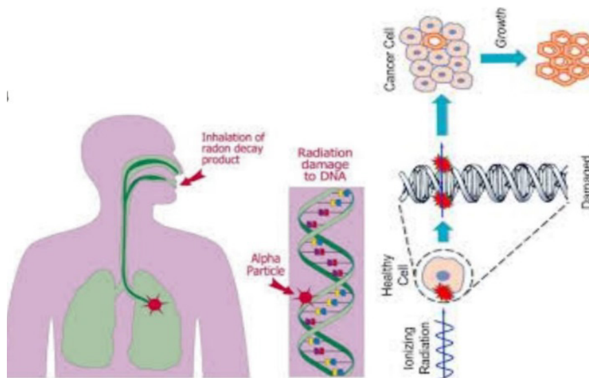
Fig. 2. Alpha particles could break some connections between bases in a DNA and produce new connections which may cause the emergence of cancer.
