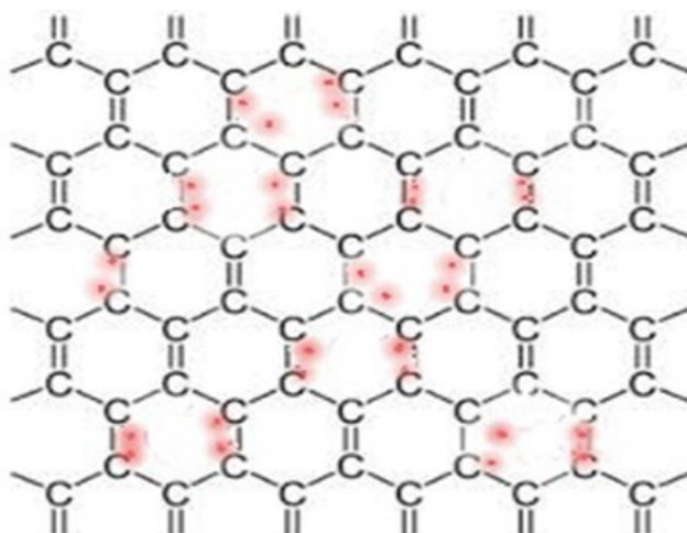
Fig. 4. A graphene sheet could have some non-paired electrons.
