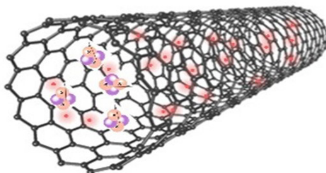
Fig. 5. Tubular graphene may have some unpaired electrons which absorb charged alpha particles.
