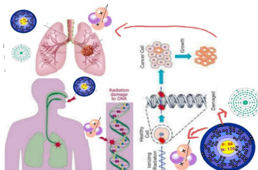
Fig. 3. Radon atoms could cause some special tumors like lung cancer.
