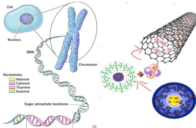
Fig. 6. Charged tubular graphene could absorb radiated alpha particles from radon atoms.
